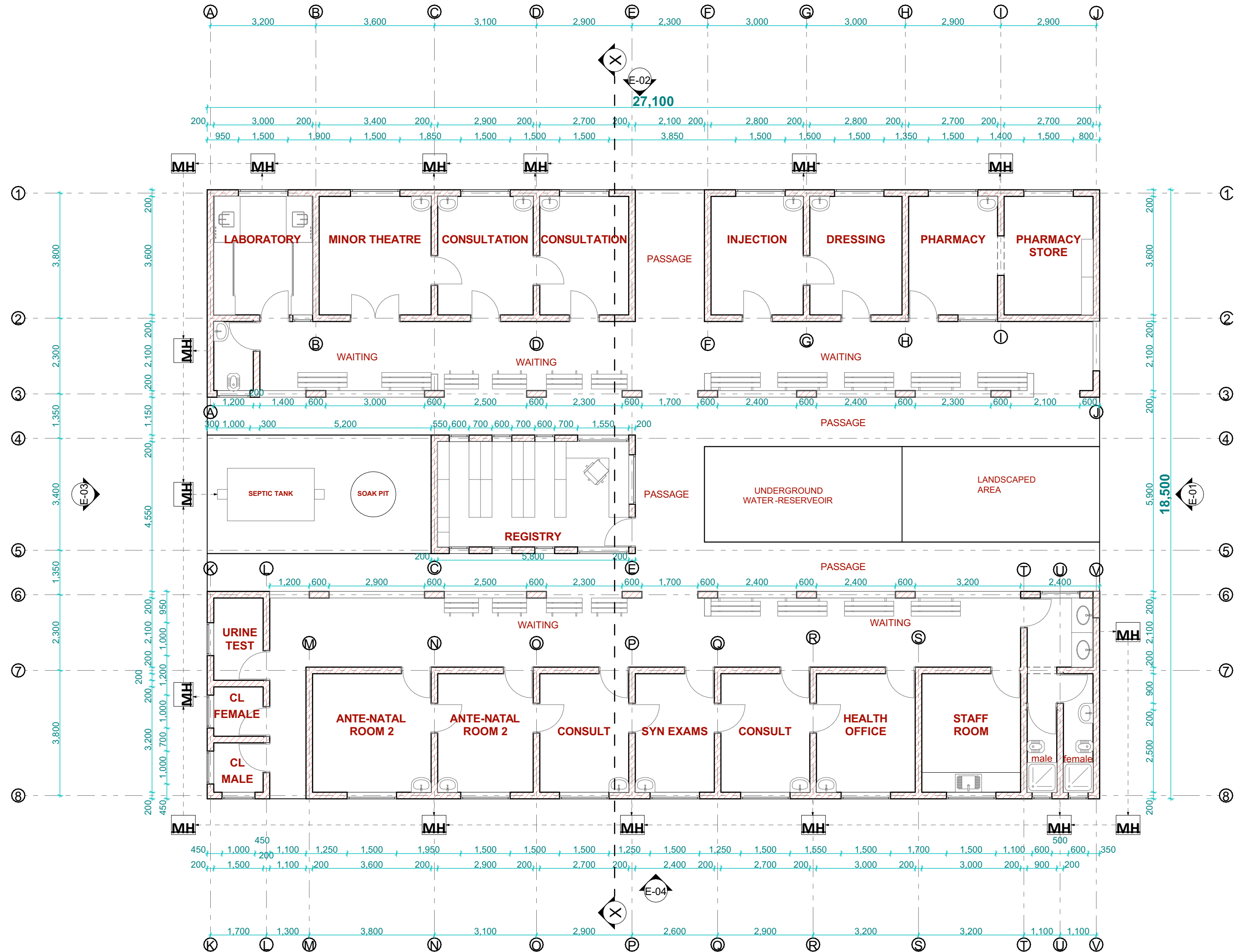
GROUND FLOOR PLAN LAYOUT - SCALE 1:100
