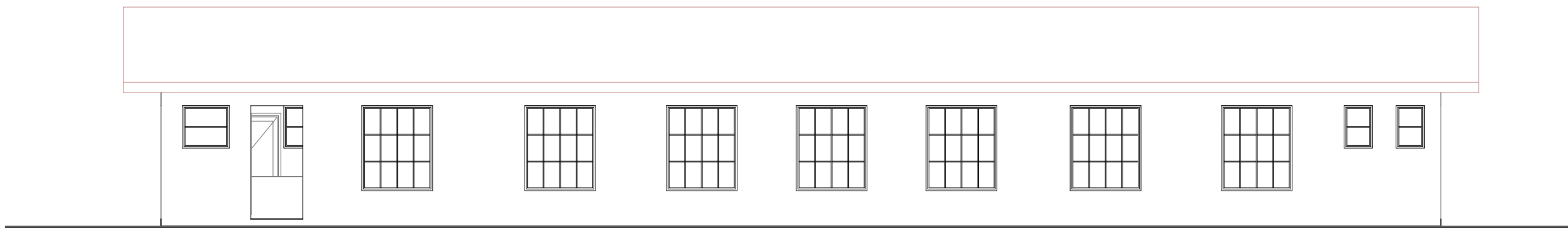
ELEVATION (03) - SCALE 1:100
