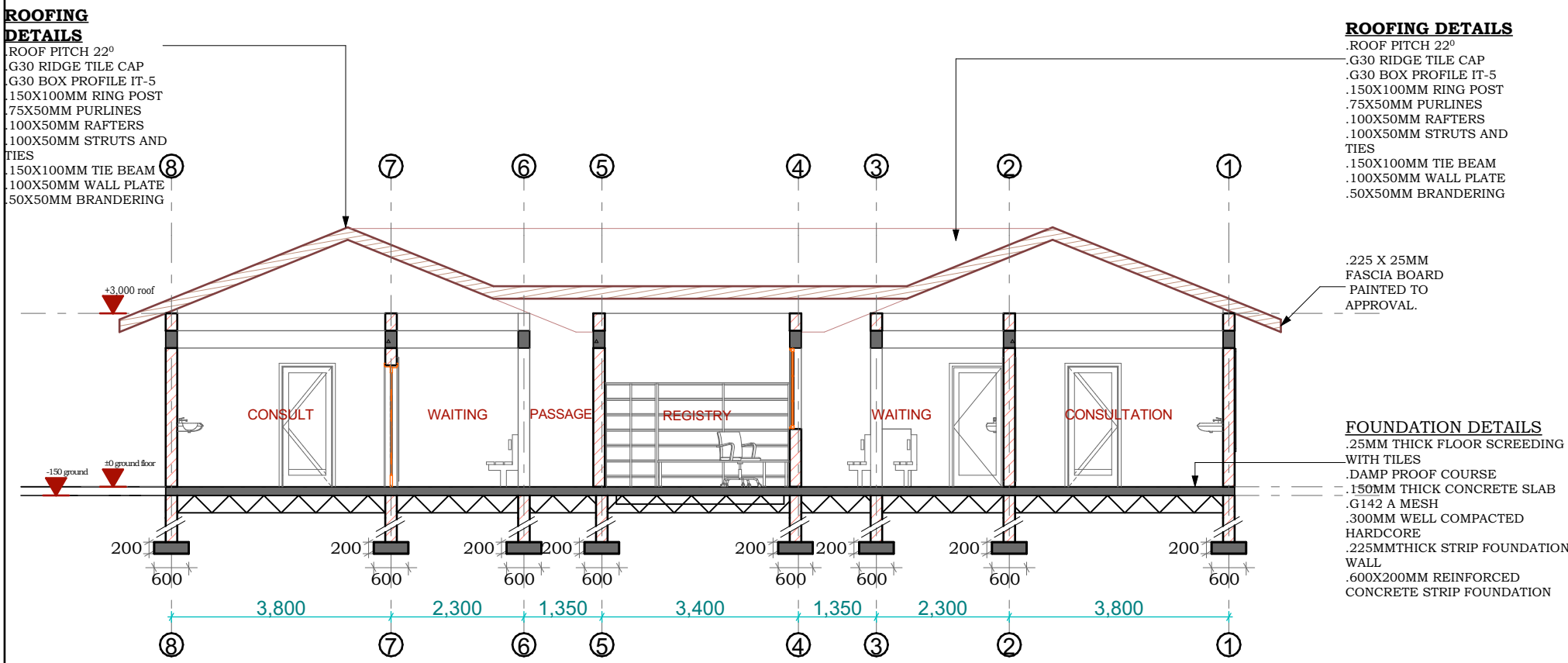
SECTION (X-X) SCALE - 1:100
