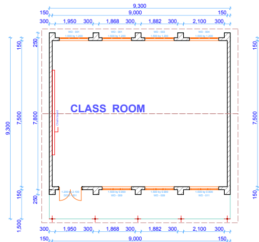
FLOOR PLAN
