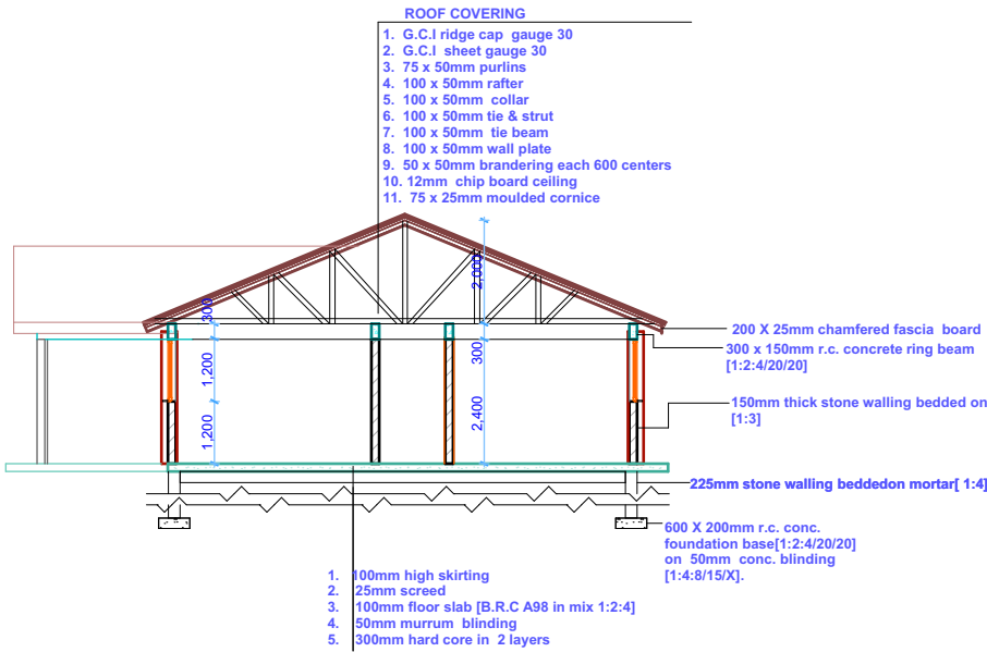
SECTION X-X
