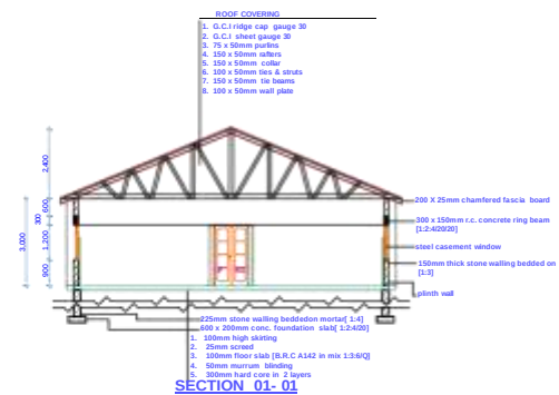
SECTION 01-01
