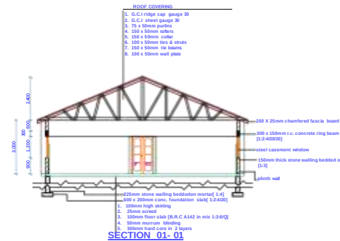
SECTION 01-01
