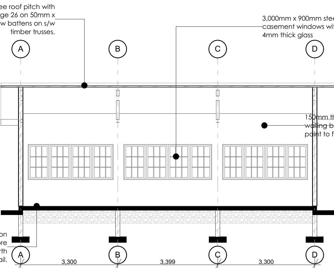
SECTION S-03 1:75
