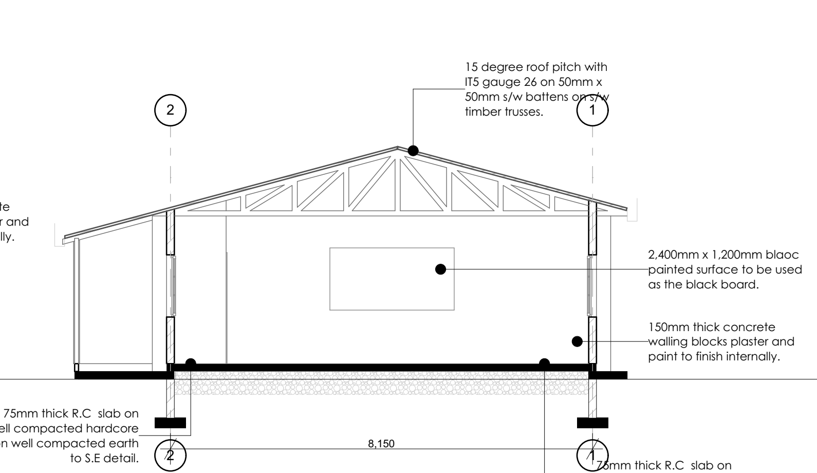
SECTION S-02 1:75
