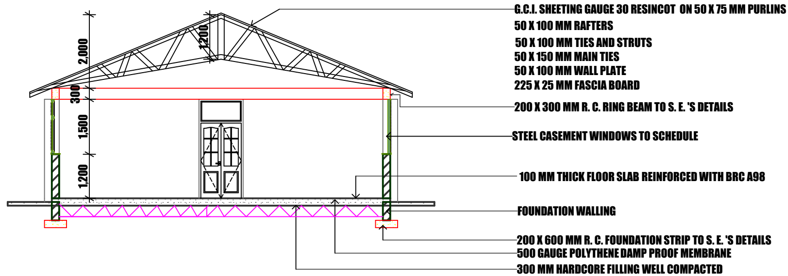
SECTION X-X
