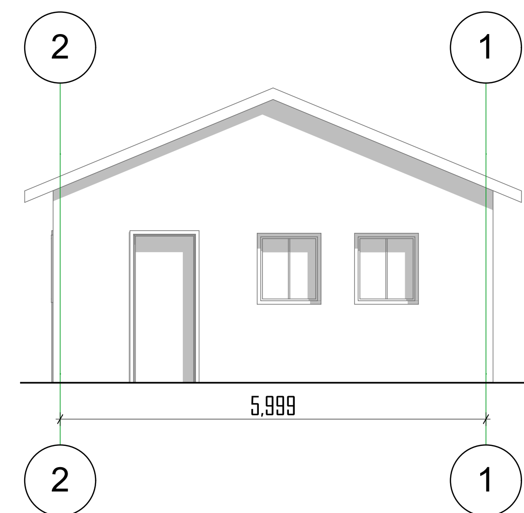
Elevation-04
