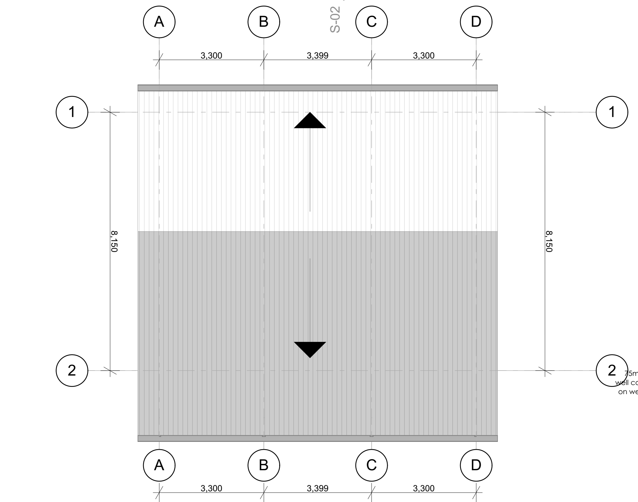
ROOF PLAN 1:75
