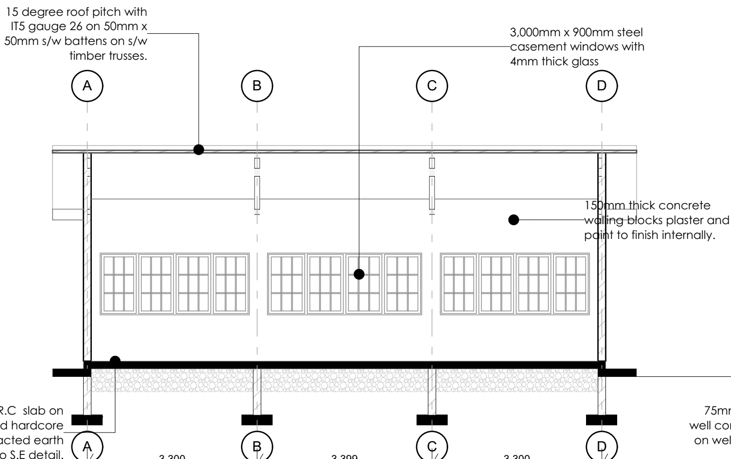
SECTION S-03 1:75
