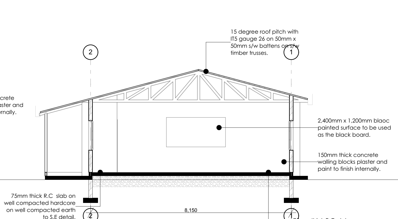
SECTION S-02 1:75
