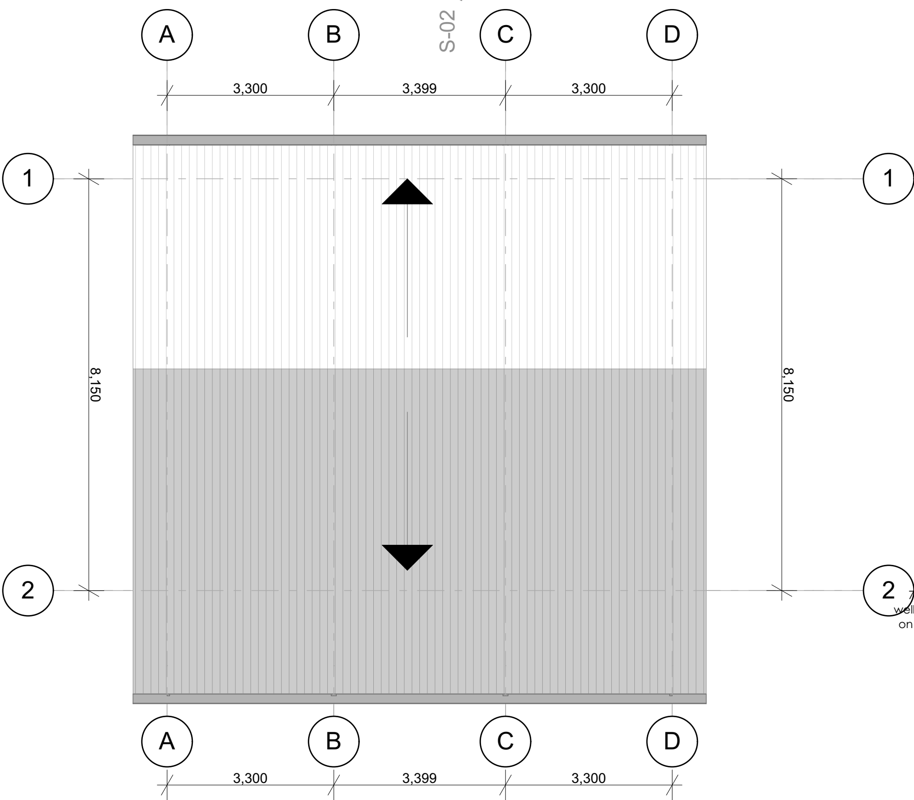
ROOF PLAN 1:75
