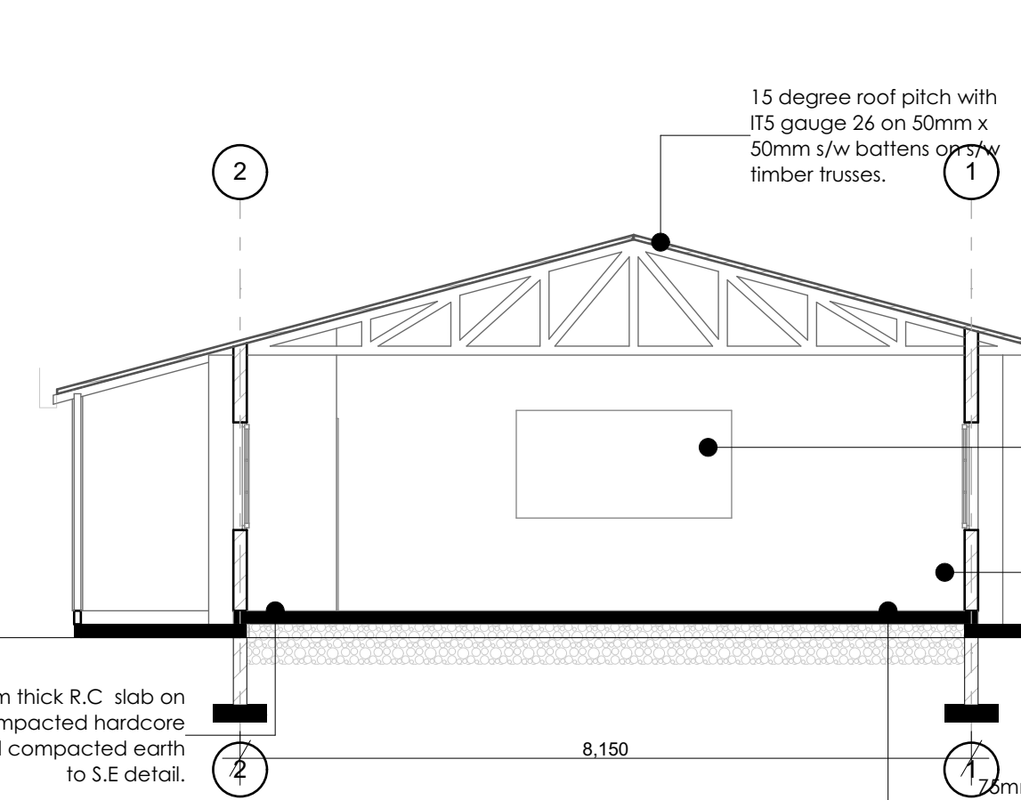
SECTION S-02 1:75
