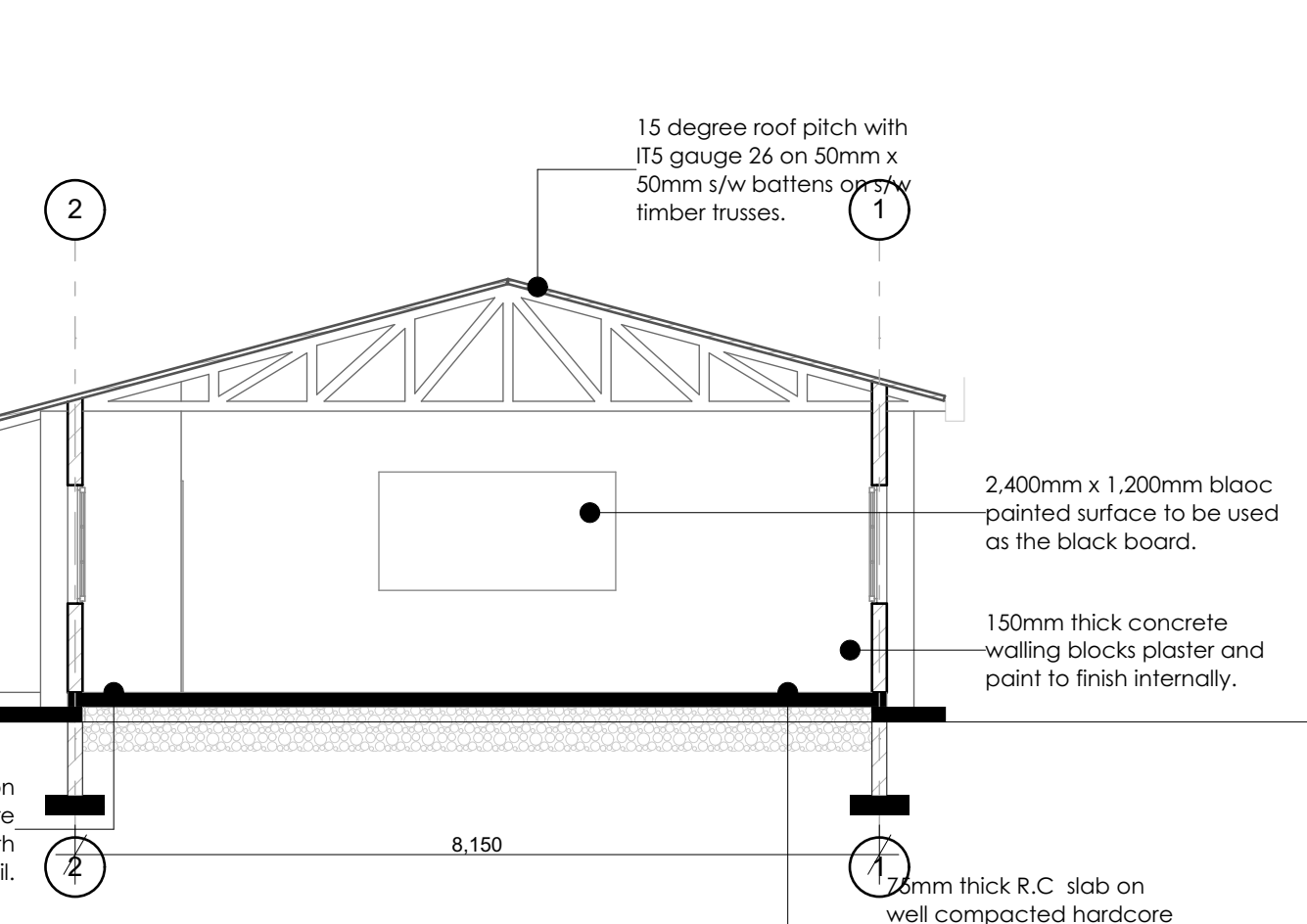
SECTION S-02 1:75
