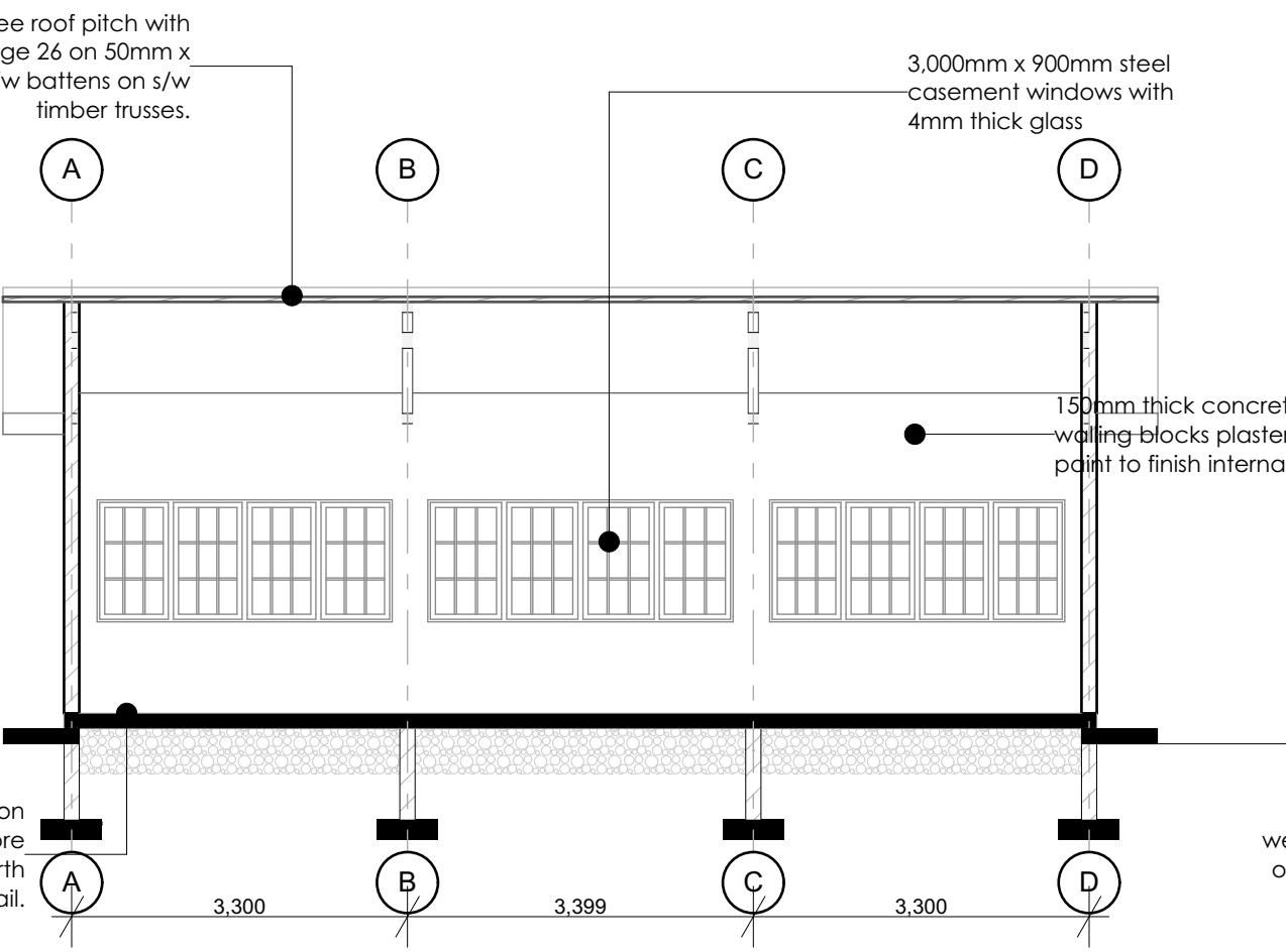
SECTION S-03 1:75
