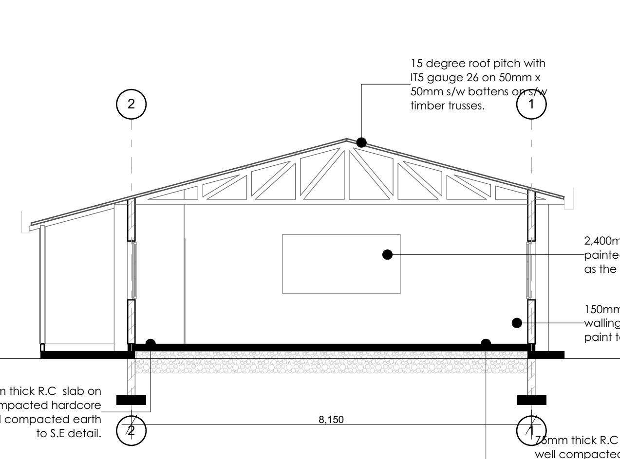
SECTION S-02 1:75
