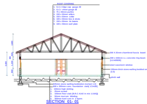
SECTION 01-01
