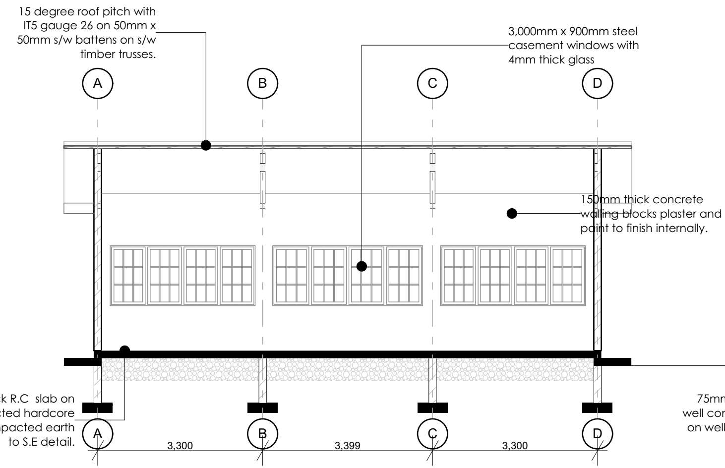
SECTION S-03 1:75
