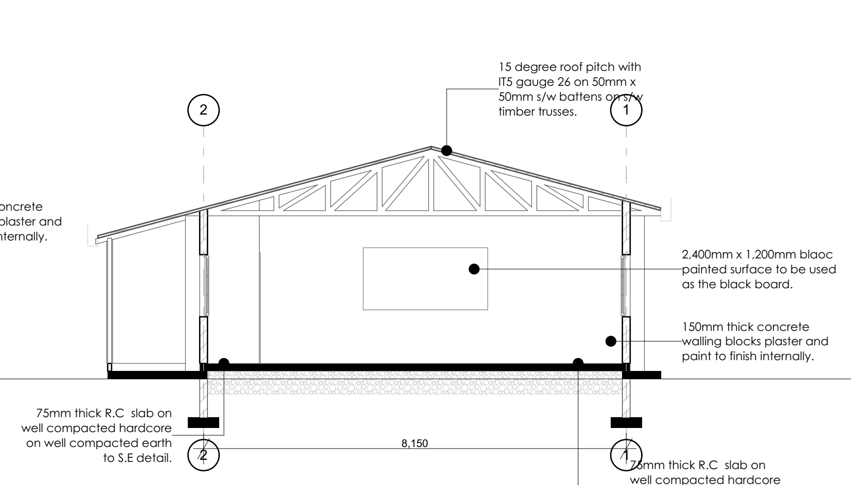
SECTION S-02 1:75
