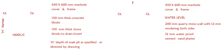
SOAK PIT DETAIL
