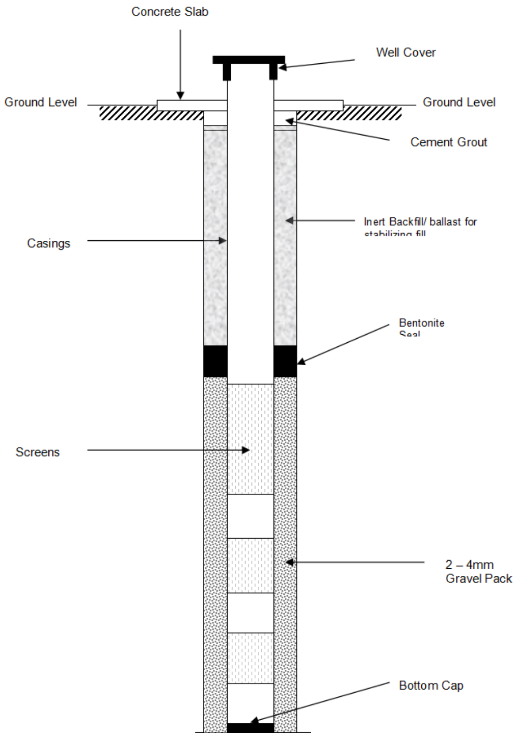
Figure 3: A representation of a completed borehole
